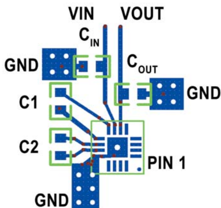
Figure 2. PCB Layout
